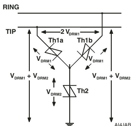
Figure 12. Off-State Voltage
