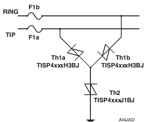
Figure 14. GR-1089-CORE Design
