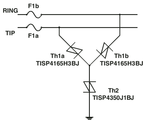
Figure 17. Asymmetrical Design for US ADSL Modems
