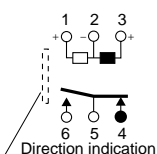
2-coil latching
