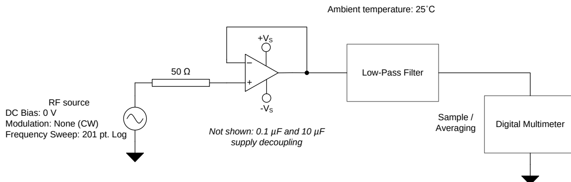
Figure 39. EMIRR +IN Test Configuration
