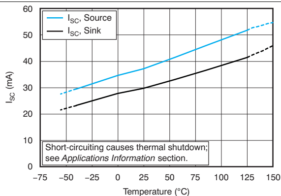
Figure 31. Short Circuit Current vs Temperature
