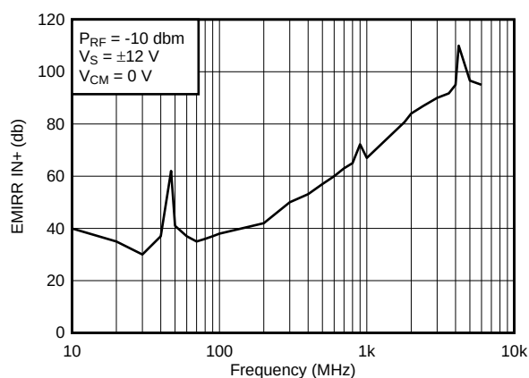
Figure 38. OPA2140 EMIRR
