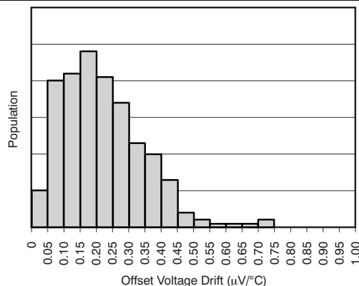
Figure 2. Offset Voltage Drift Distribution
