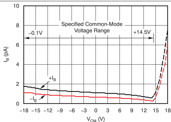
Figure 5. I_B vs Common-Mode Voltage
