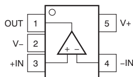
DBV Package: OPA140 5-Pin SOT-23 Top View
