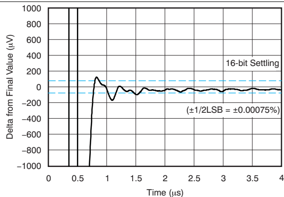
Figure 25. Large-Signal Positive Settling Time (10-V Step)
