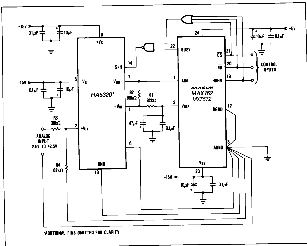
Figure 16. MAX162/MX7572—HA5320 Sample-and-Hold Interface
