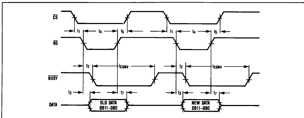
Figure 12. ROM Mode, Parallel Read Timing Diagram
