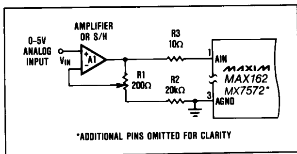
Figure 18. Full-Scale Adjustment
