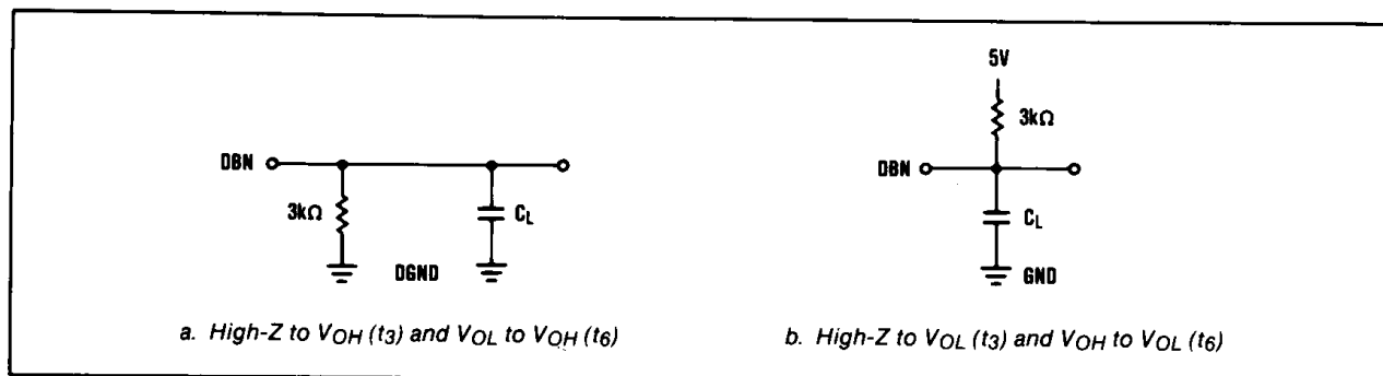
Figure 1. Load Circuits for Access Time
