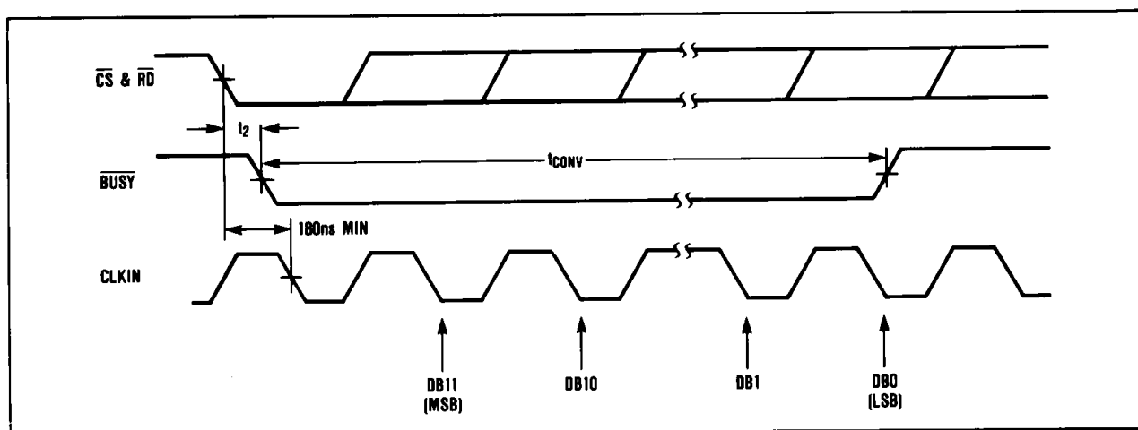
Figure 8. MX7572 \overline{RD} and CLKIN For Synchronous Operation
