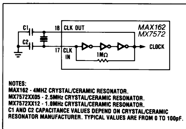
Figure 6. MAX162/MX7572 Internal Clock Circuit
