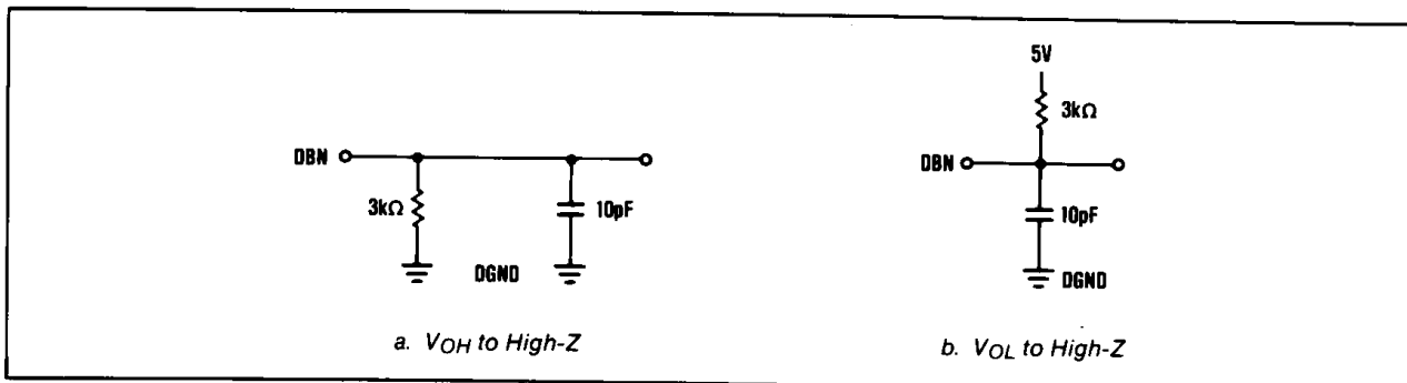
Figure 2. Load Circuits for Output Float Delay
