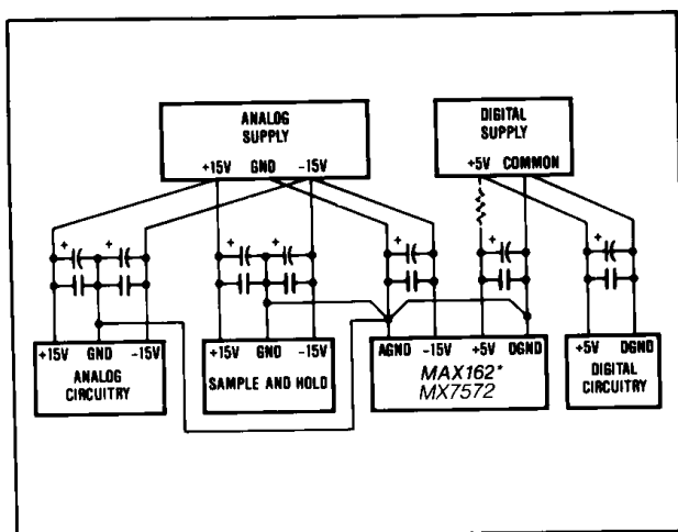
Figure 14. Power Supply Grounding Practice
