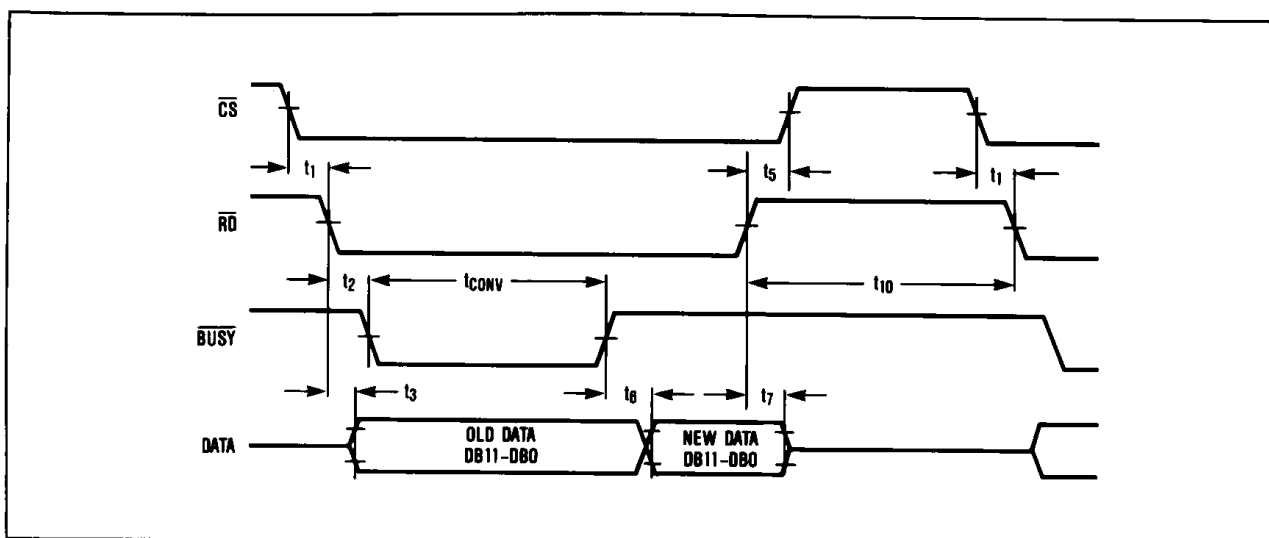
Figure 10. Slow Memory Mode, Parallel Read Timing Diagram
