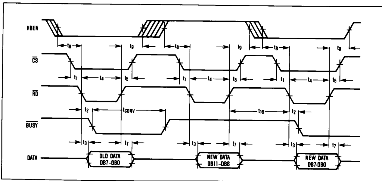
Figure 13. ROM Mode, Two Byte Read Timing Diagram
