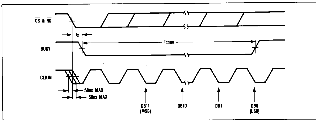
Figure 7. MAX162 \overline{RD} and CLKIN For Synchronous Operation
