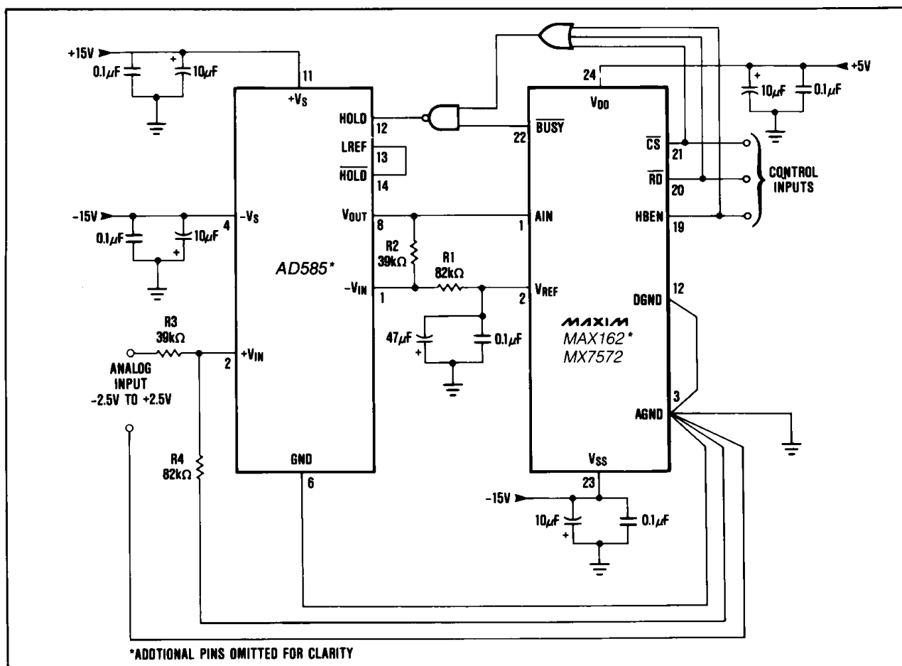
Figure 15. MX7572—AD585 Sample-and-Hold Interface
