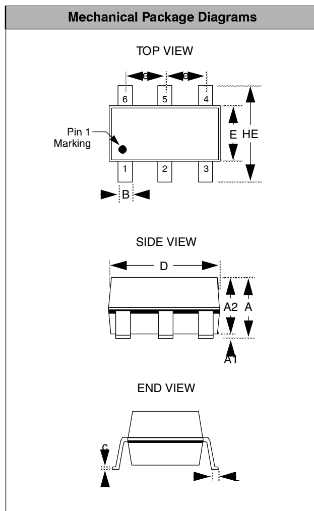
Package Dimensions for SC70-6.
