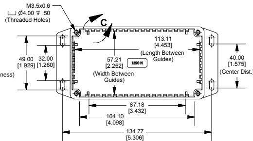
DETAIL C Top View - Interior Features
