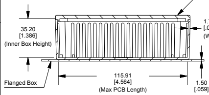
SECTION B-B Side View of Assembly
