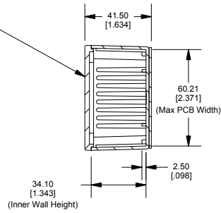
SECTION A-A End View of Assembly
