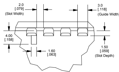
DETAIL C Top View - Interior Features
