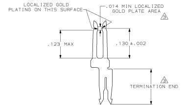
DETAIL Z SCALE 10:1 TYPICAL
