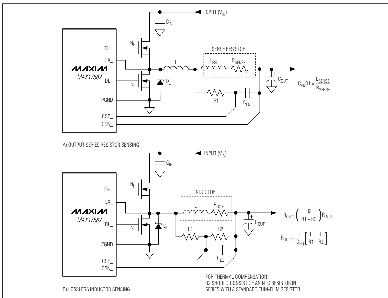
Figure 3. Current-Sense Methods
