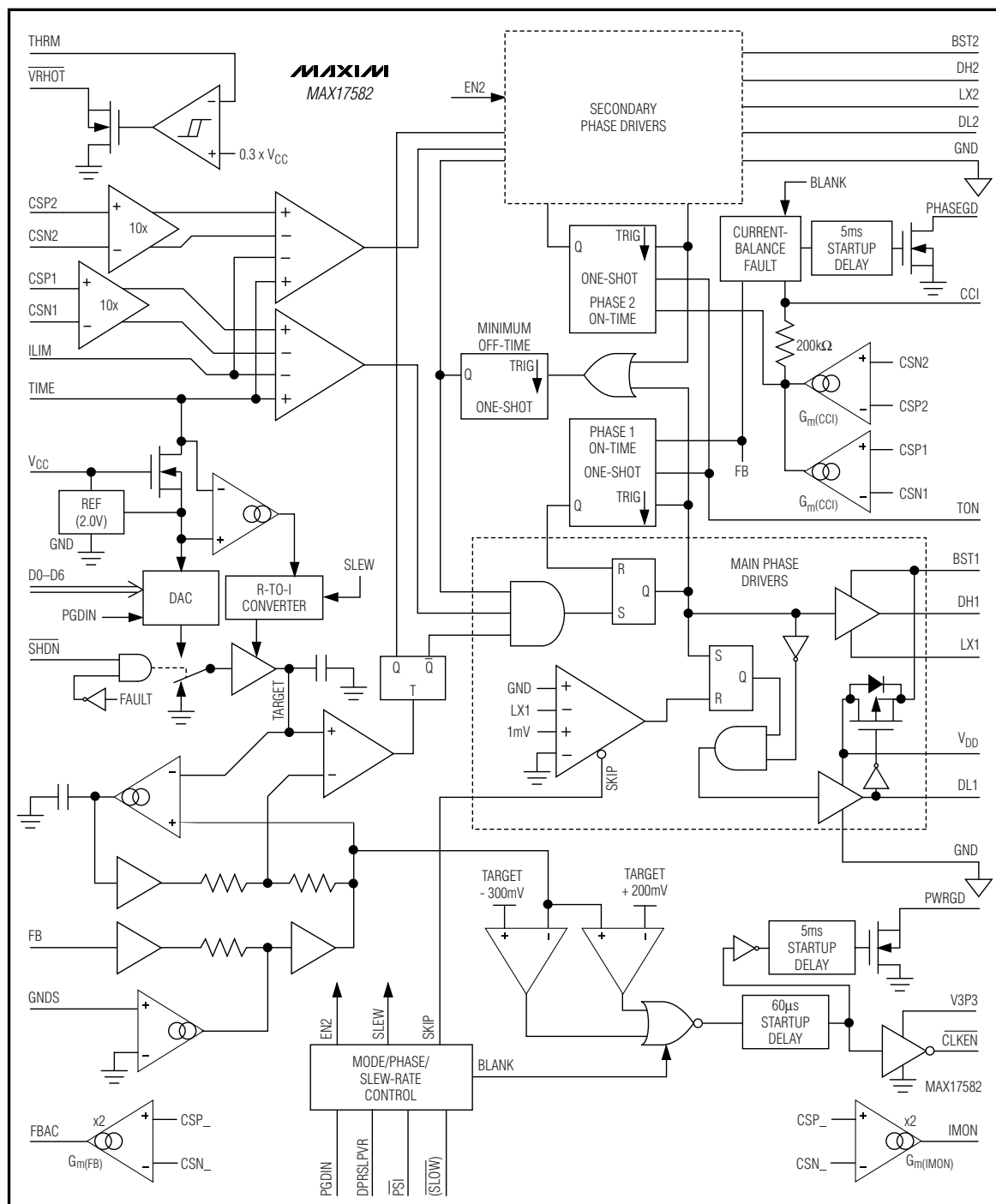
Figure 2. Functional Diagram
