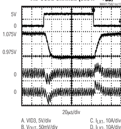
VID CODE CHANGE (SLOW = V_{DD} )
