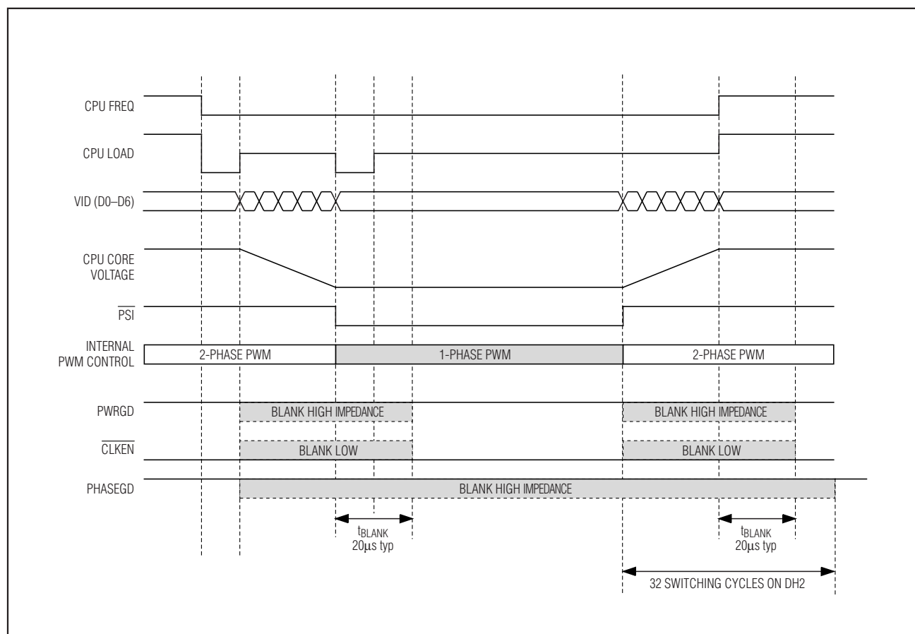
Figure 6. \overline{\text{PSI}} Transition
