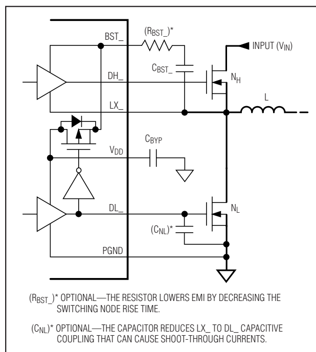
Figure 9. Gate Drive Circuit
