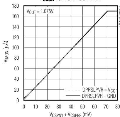
V_{MON} vs. LOAD CURRENT
