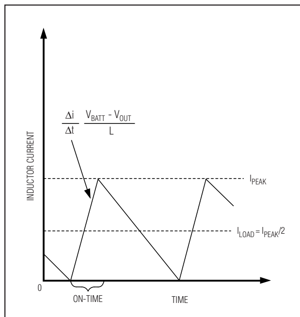
Figure 7. Pulse-Skipping/Discontinuous Crossover Point
