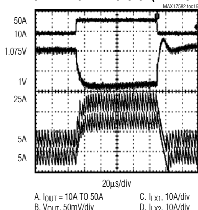
LOAD-TRANSIENT RESPONSE (HFM MODE)
