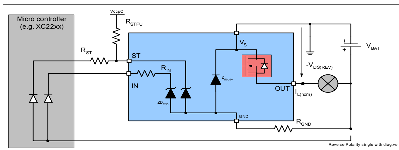
Figure 9 Reverse polarity protection with external components
