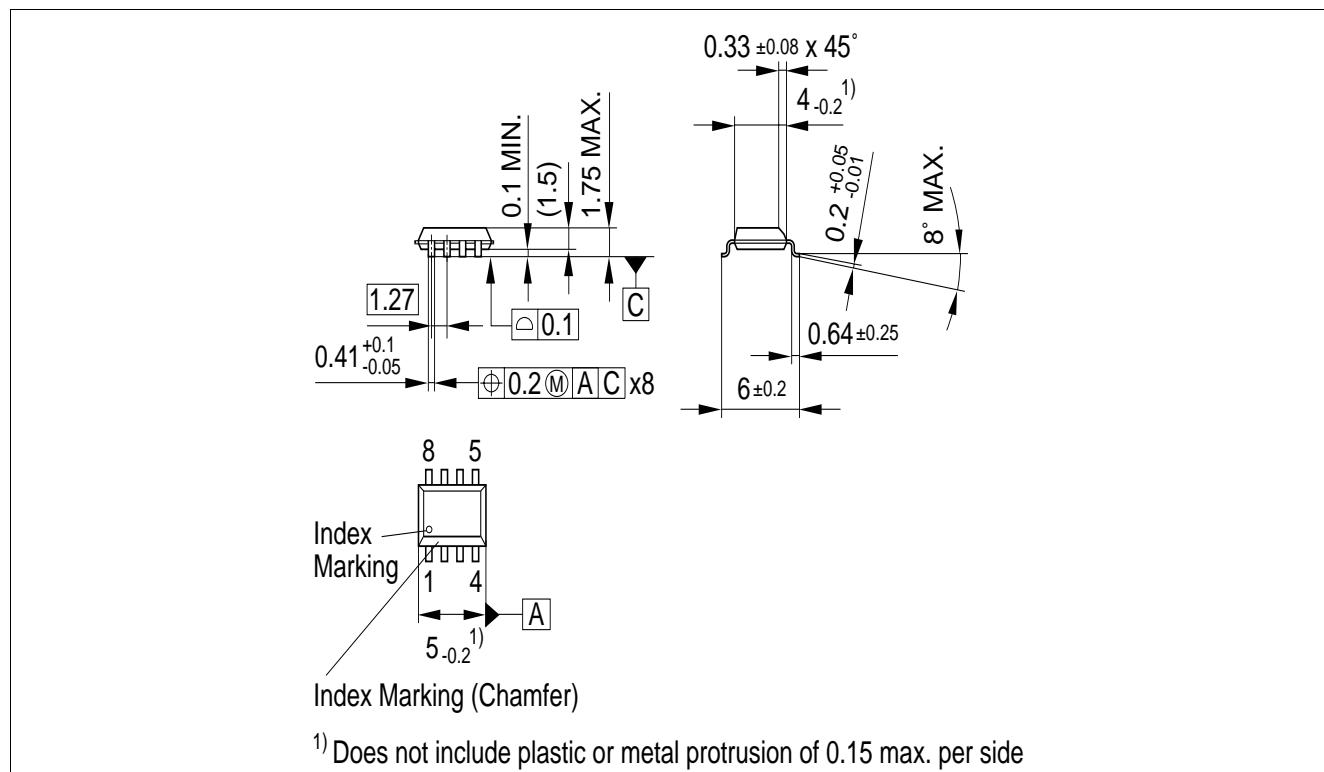
Figure 17 PG-DSO-8-24 (Plastic Dual Small Outline Package)
