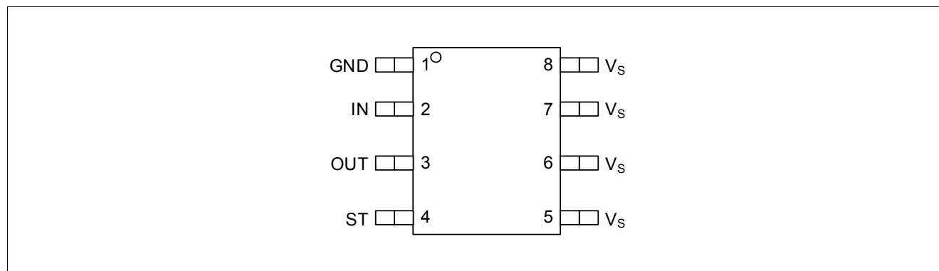
Figure 2 Pin Configuration
