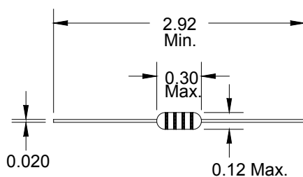
Dimensions: Inches
