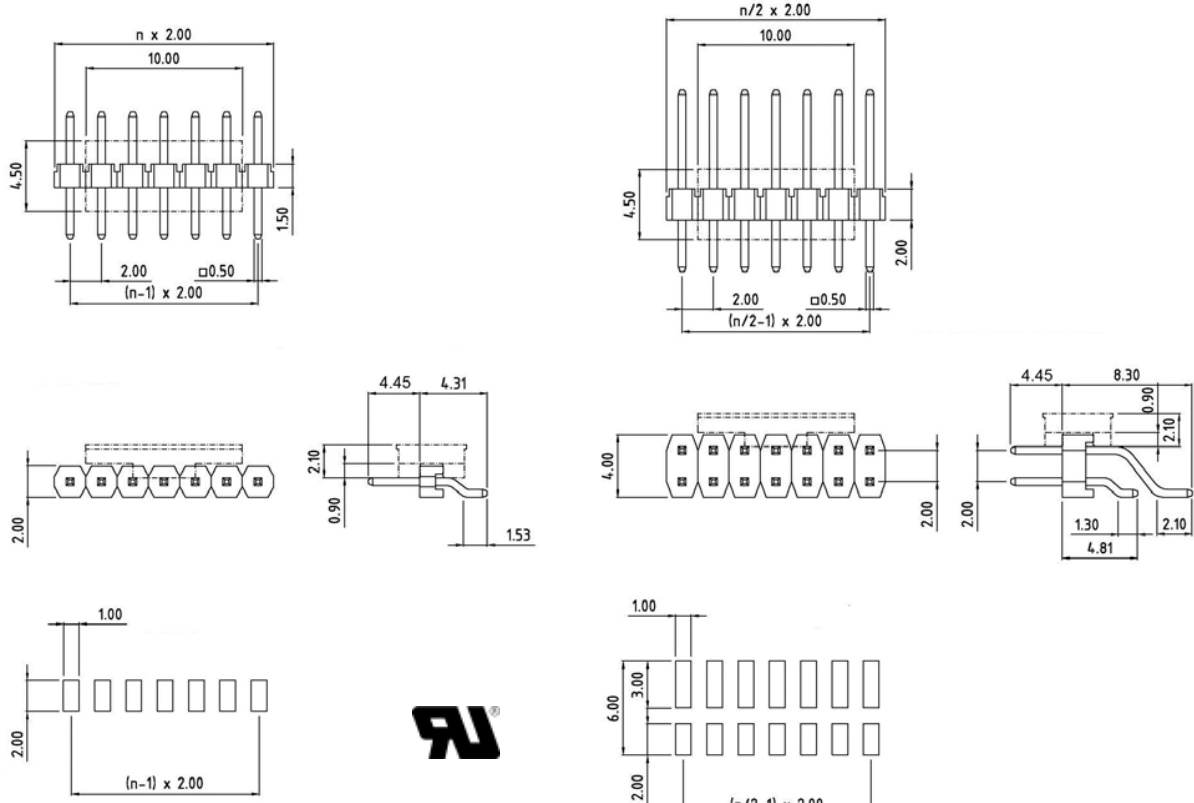
PCB-Layout
