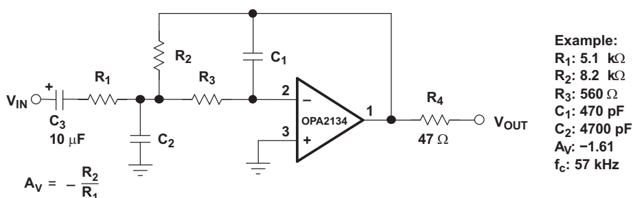
Figure 33. Dual-Supply Filter Circuit
