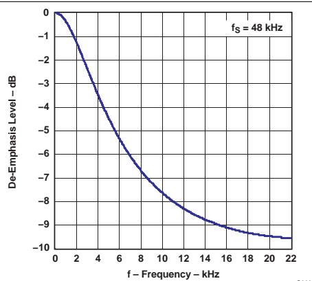
Figure 10. De-Emphasis
