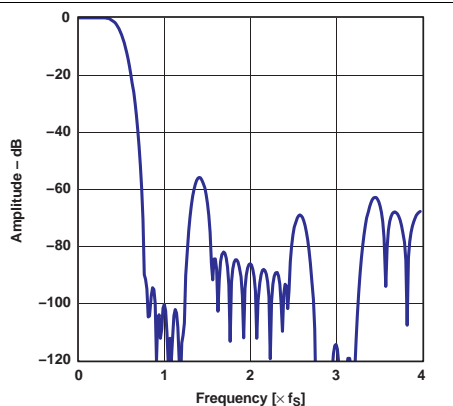
Figure 4. Frequency Response (Slow Roll-off)
