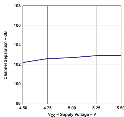
Figure 16. Channel Separation vs Supply Voltage
