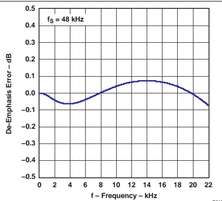
Figure 11. De-Emphasis Error
