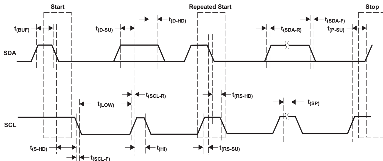
Figure 1. Interface Timing
