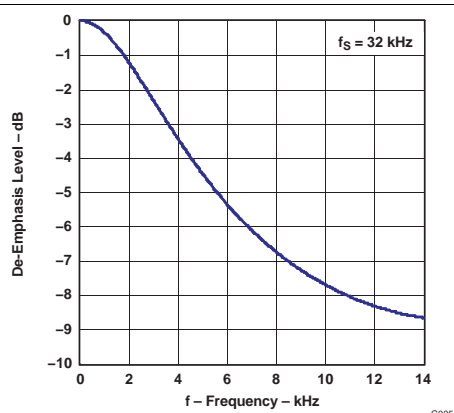
Figure 6. De-Emphasis
