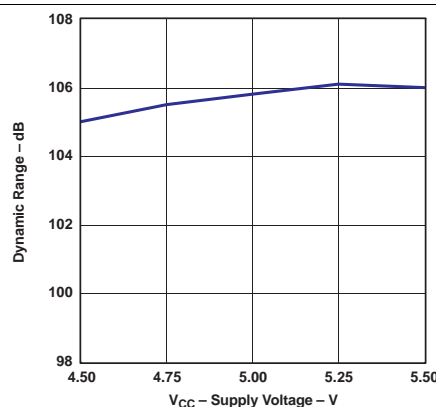
Figure 14. Dynamic Range vs Supply Voltage
