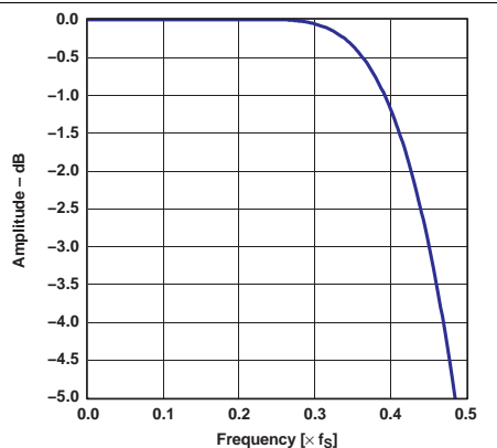
Figure 5. Transition Characteristics (Slow Roll-off)
