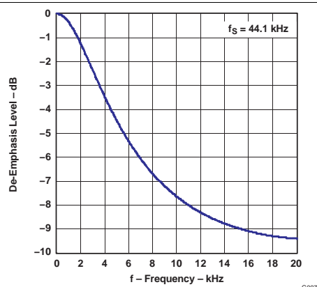
Figure 8. De-Emphasis
