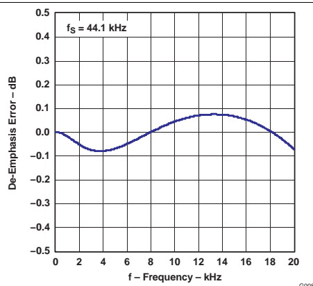
Figure 9. De-Emphasis Error
