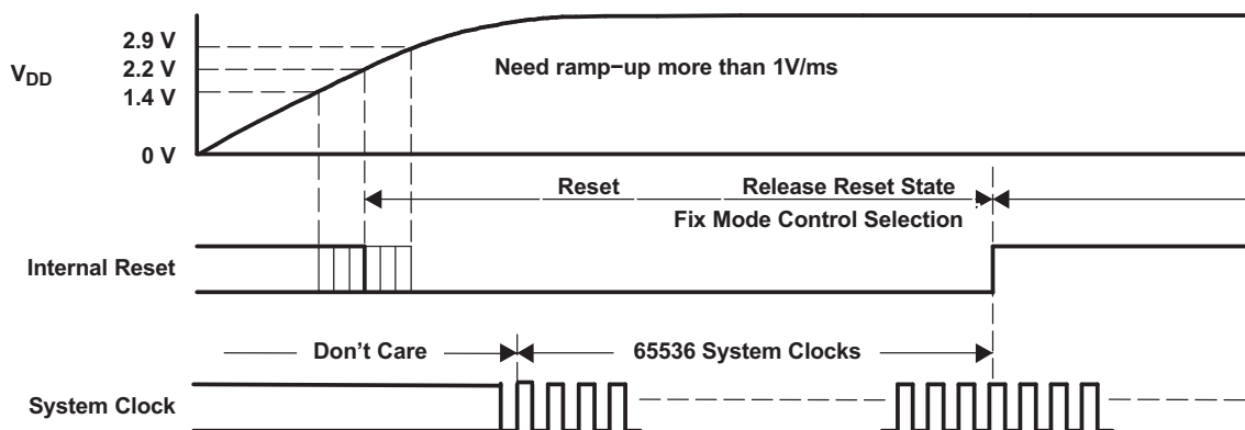
Figure 22. Power-On-Reset Timing
