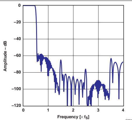
Figure 2. Frequency Response (Sharp Roll-off)
