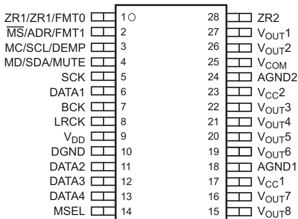
Pin Functions
