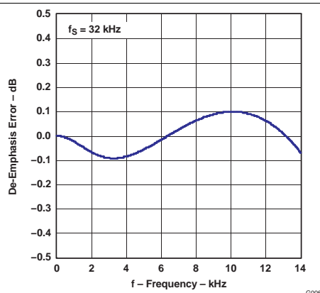
Figure 7. De-Emphasis Error
