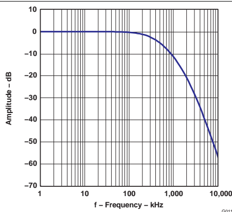
Figure 12. Analog Filter Performance
