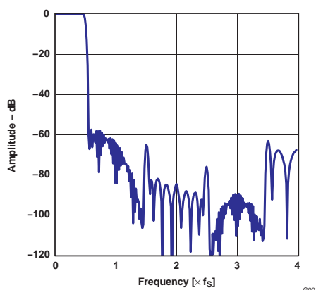
Figure 35. Frequency Response (Sharp Roll-off)
