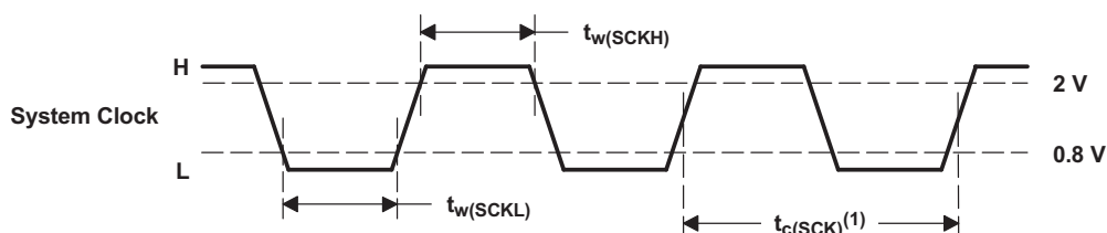
Figure 21. System Clock Timing Diagram
