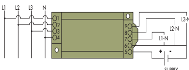
CR4870 3 Element, 4 Wire - 0 - 5 VDC Output
