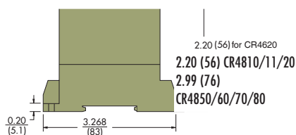
Dimensions for Models CR4850, 4860, 4870, 4880 (shown)
