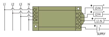
CR4880 3 Element, 4 Wire - 4 - 20 mA DC Output
