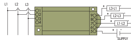
CR4860 3 Element, 3 Wire - 4-20 mA DC Output
