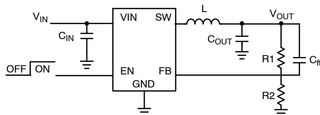
Figure 1. Typical Application for Adjustable Version
