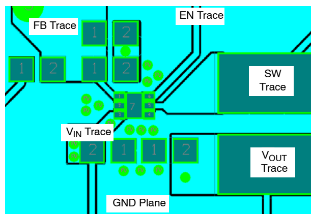
Figure 31. UDFN6 Recommended Board Layout
