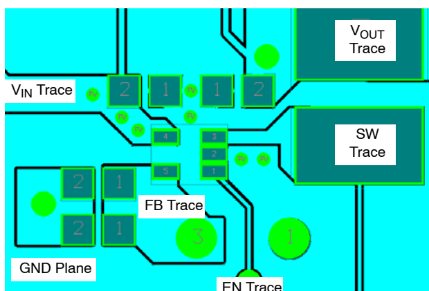
Figure 30. TSOP-5 Recommended Board Layout
