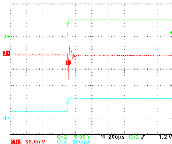
Figure 18. 200 mA to 600 mA Load Transient in 1\text{ }\mu\text{s} ( V_{IN} = 3.6\text{ V} , V_{OUT} = 1.2\text{ V} , Temperature = 25^{\circ}\text{C} )
