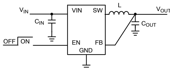
Figure 2. Typical Application for Fixed Version
