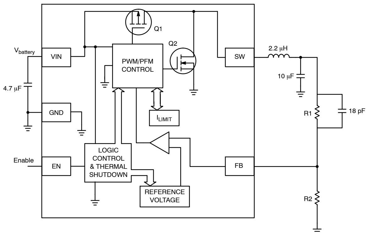
Figure 6. Simplified Block Diagram
