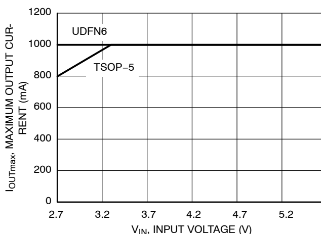
Figure 7. Maximum Output Current, T_A = 45^\circ\text{C}
