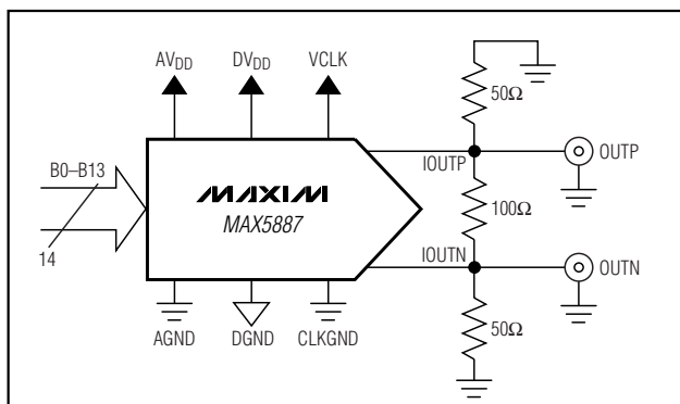
Figure 8. MAX5887 Differential Output Configuration
