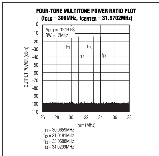
Figure 12. Four-Tone MTPR Test Results
