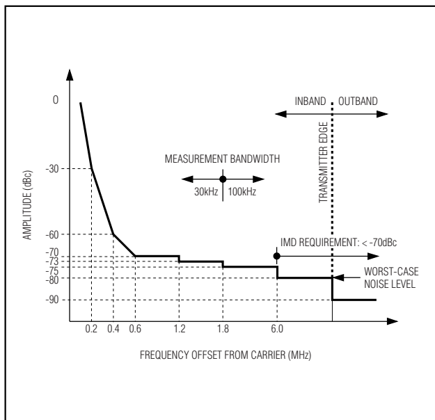
Figure 11. GSM/EDGE Tx Mask Requirements
