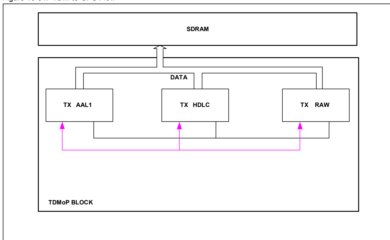
Figure 10-54. TDM-to-CPU Flow
