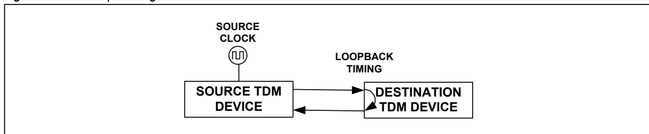
Figure 10-46. Loop Timing in TDM Networks
