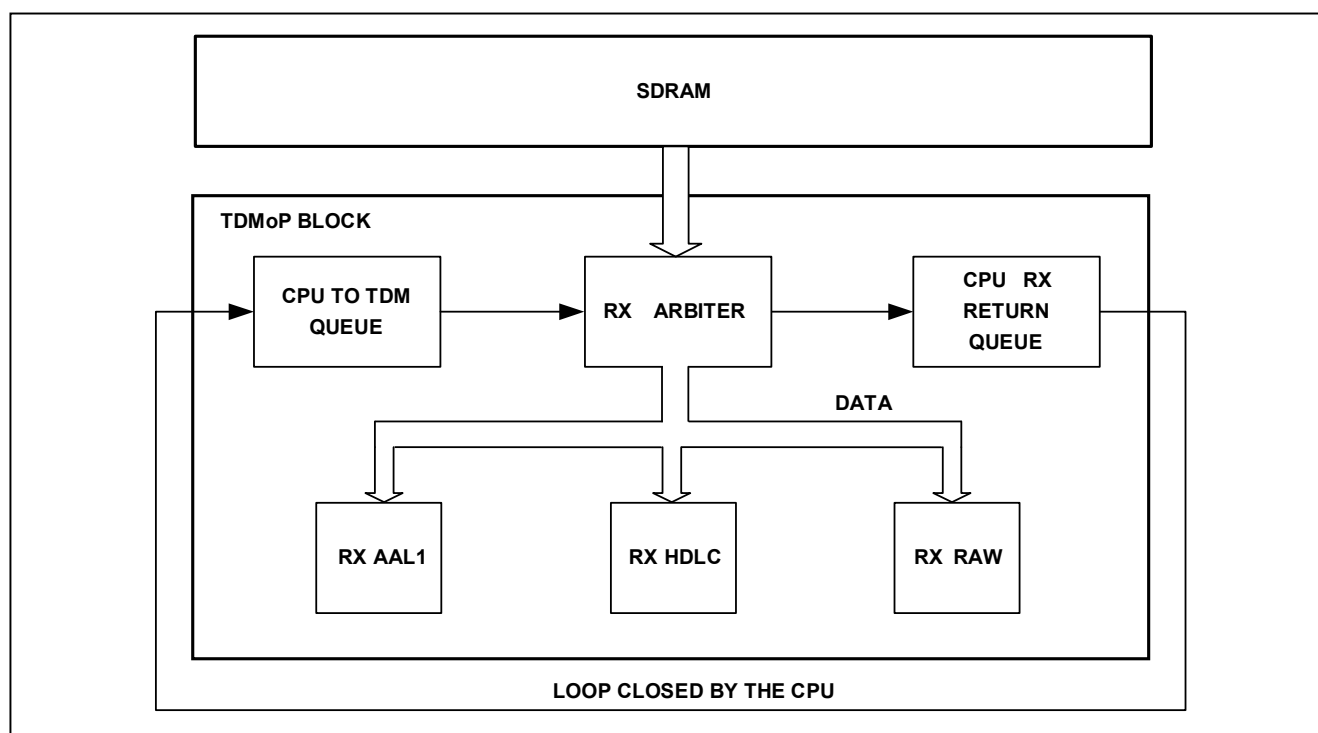
Figure 10-55. CPU-to-TDM Flow
