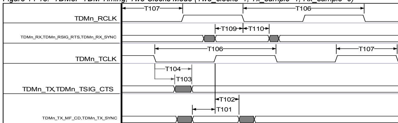
Figure 14-13. TDMoP TDM Timing, Two Clocks Mode (Two_clocks=1, Tx_sample=1, Rx_sample=0)
