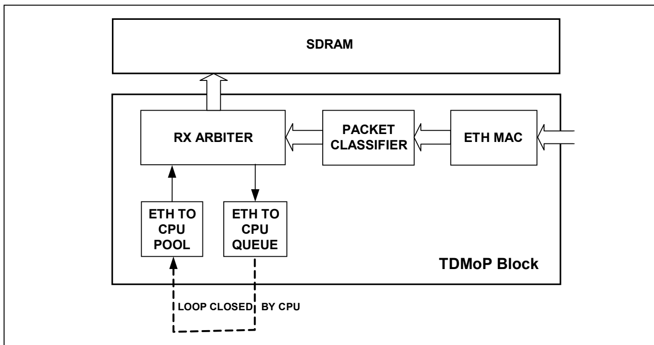
Figure 10-57. Ethernet-to-CPU Flow
