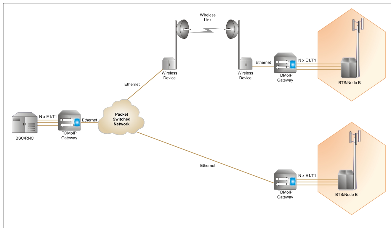
Figure 5-2. TDMoP in Cellular Backhaul
