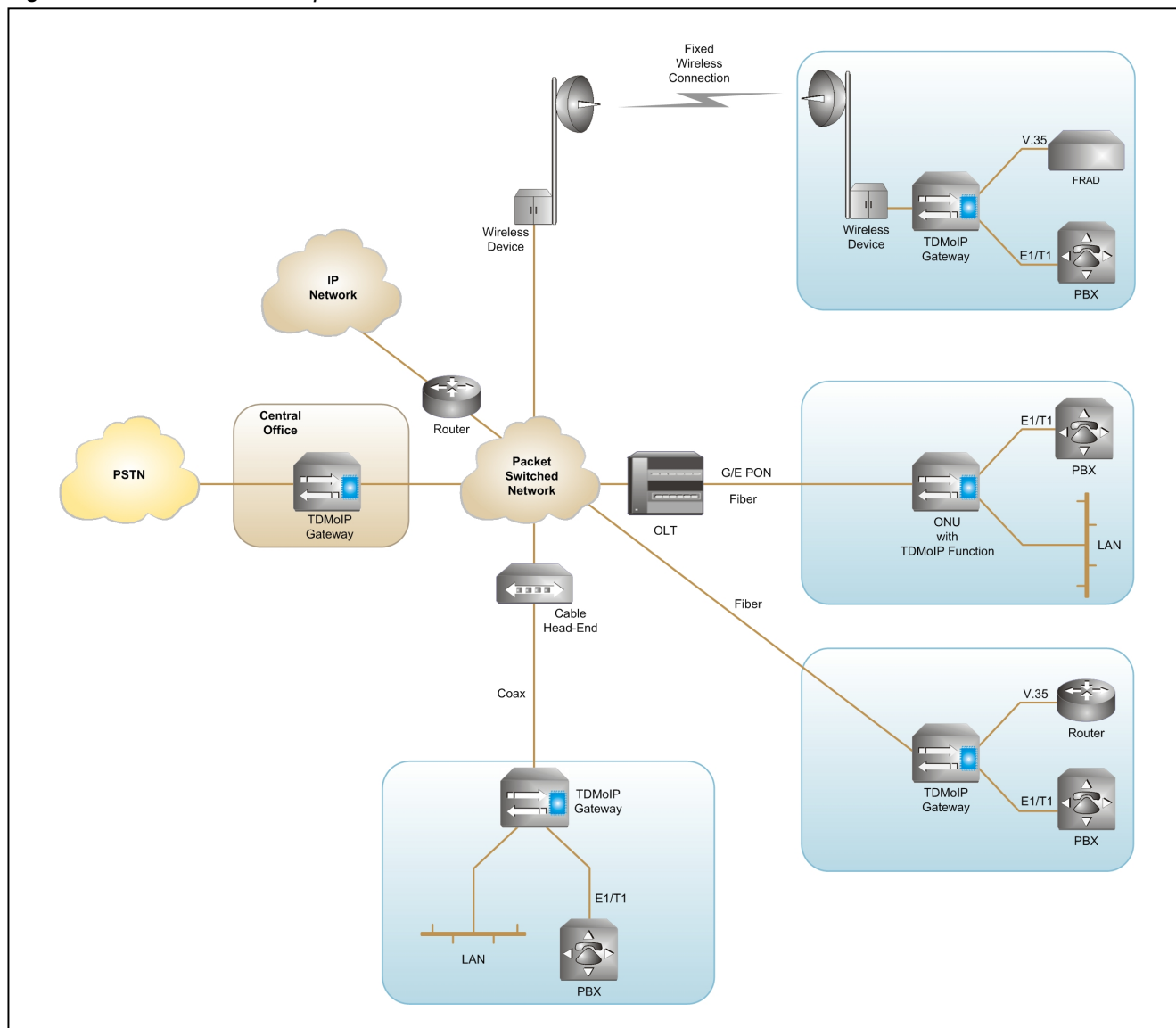
Figure 5-1. TDMoP in a Metropolitan Packet Switched Network
