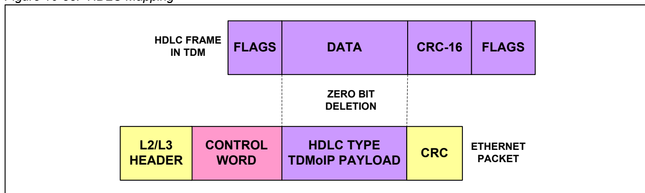
Figure 10-38. HDLC Mapping
