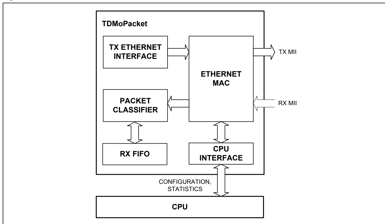
Figure 10-58. Ethernet MAC
