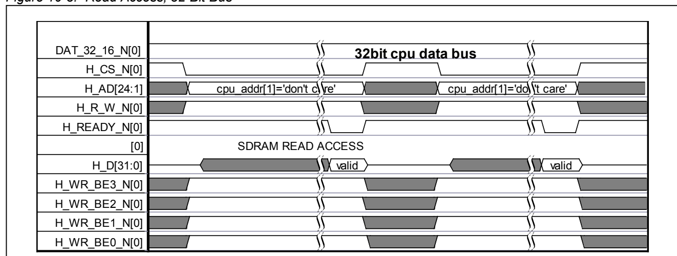
Figure 10-3. Read Access, 32-Bit Bus
