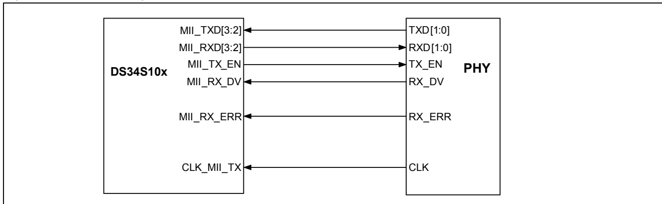
Figure 15-4. Connecting the Ethernet Port to a PHY in RMII Mode
