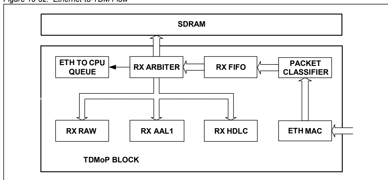
Figure 10-52. Ethernet-to-TDM Flow
