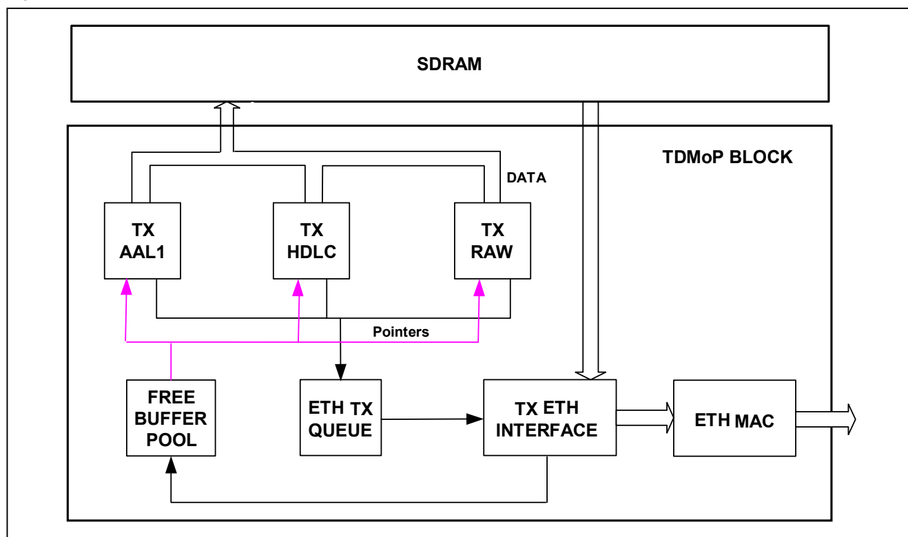
Figure 10-51. TDM-to-Ethernet Flow
