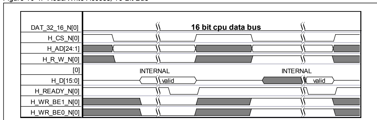
Figure 10-4. Read/Write Access, 16-Bit Bus
