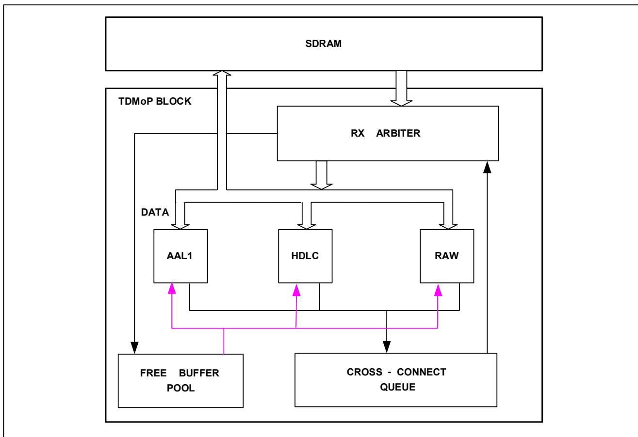
Figure 10-53. TDM-to-TDM Flow
