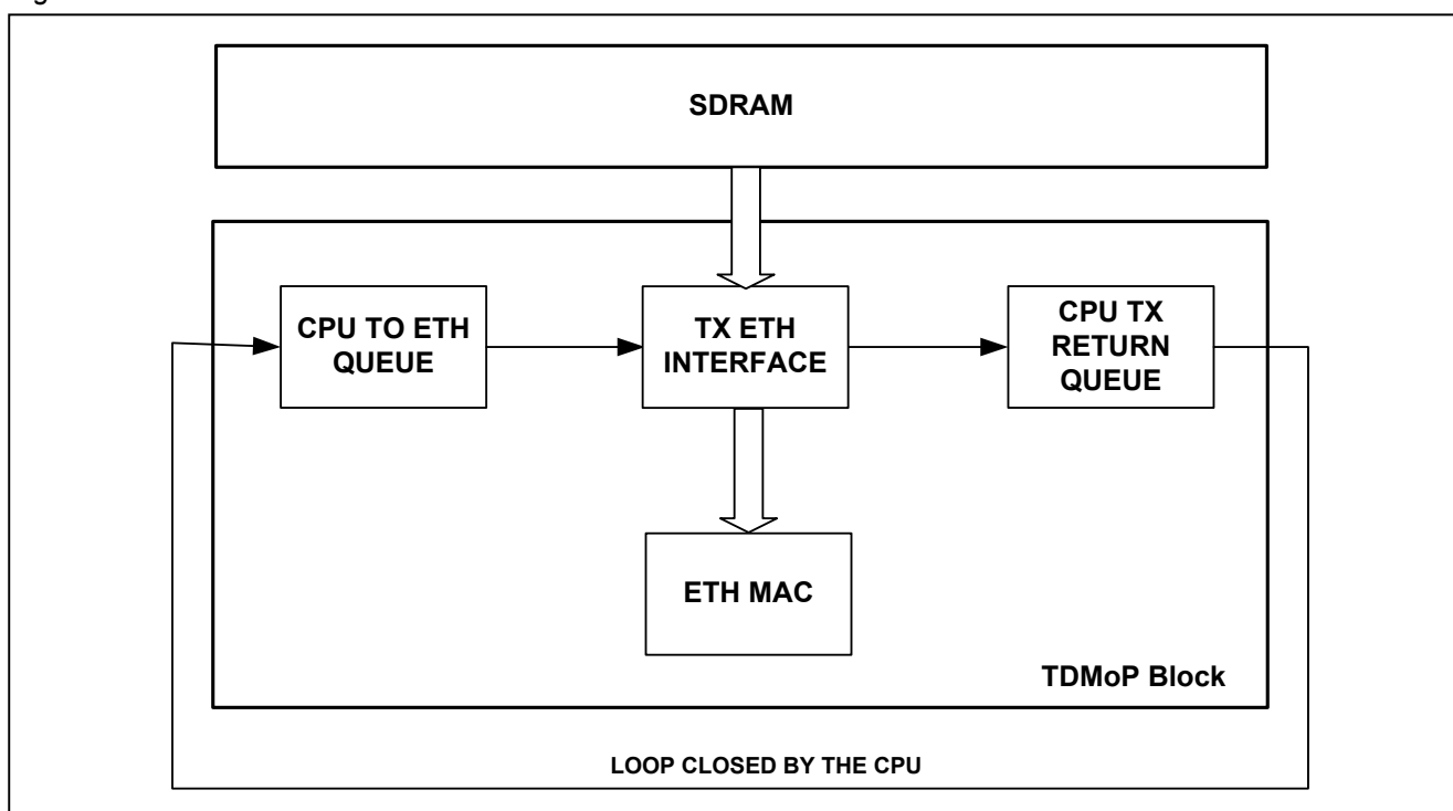
Figure 10-56. CPU-to-Ethernet Flow
