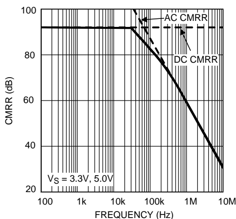
Figure 50. CMRR Curve
