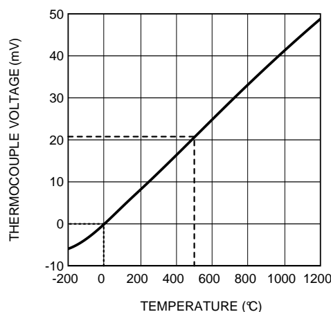
Figure 56. K-Type Thermocouple Response
