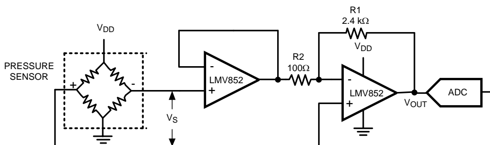
Figure 55. Pressure Sensor Application
