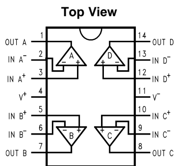
Figure 4. 14-Pin TSSOP Package See Package Number PW0014A
