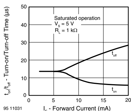
Fig. 15 - Turn-on/off Time vs. Forward Current
