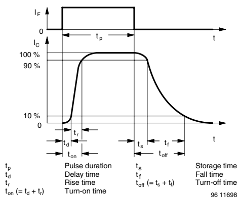
Fig. 5 - Switching Times
