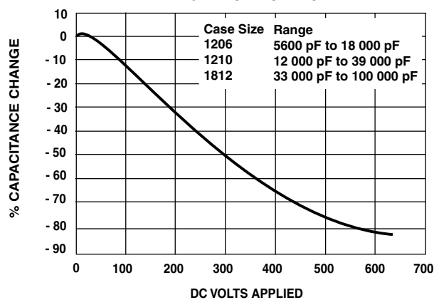
VOLTAGE COEFFICIENT OF CAPACITANCE HIGHER CAPACITANCE
