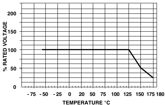
RATED VOLTAGE VS. TEMPERATURE
