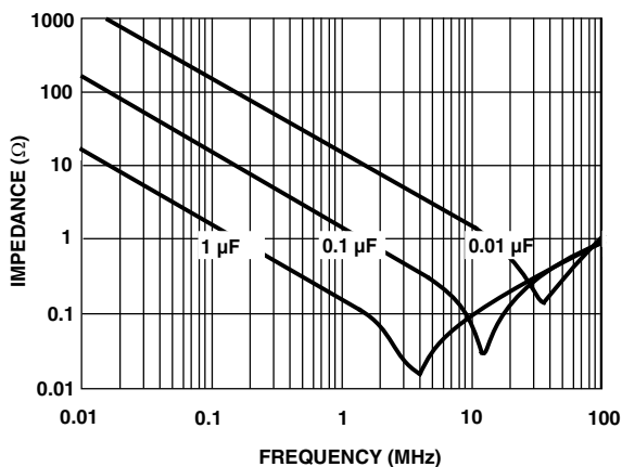
IMPEDANCE VS. FREQUENCY 500 V/630 V
