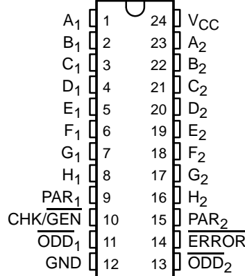
CY54FCT480T . . . L PACKAGE (TOP VIEW)
