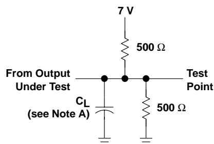
LOAD CIRCUIT FOR OPEN-DRAIN OUTPUTS
