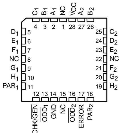
CY54FCT480T . . . L PACKAGE (TOP VIEW)
