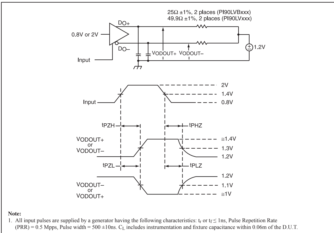
Figure 5. Enable & Disable Time Circuit & Definitions
