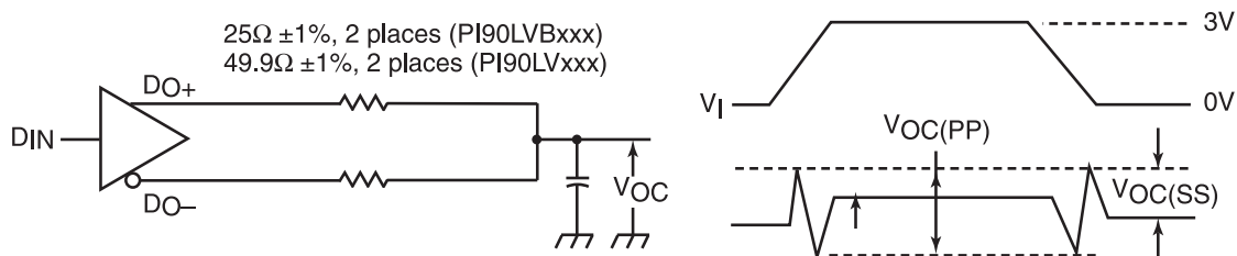
Figure 3. Test Circuit & Definitions for the Driver Common-Mode Output Voltage
