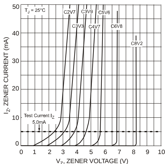
Fig. 2 Typical Zener Breakdown Characteristics
