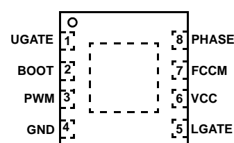
ISL6208BCRZ, ISL6208BIRZ (8 LD 2x2 DFN) TOP VIEW
