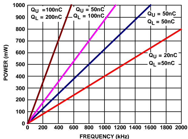
FIGURE 9. POWER DISSIPATION vs FREQUENCY
