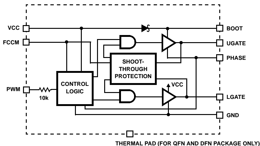
FIGURE 1. BLOCK DIAGRAM
