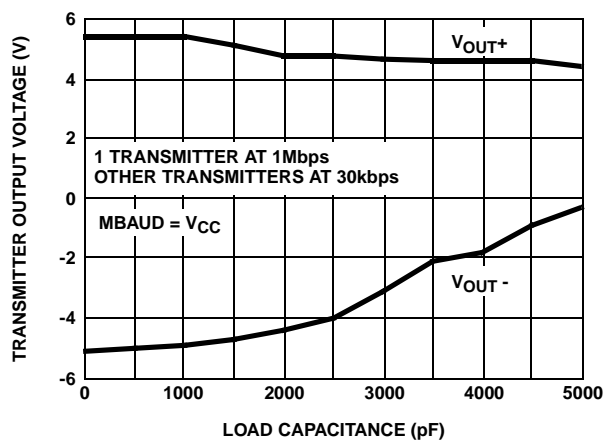
FIGURE 9. HIGH SPEED TRANSMITTER OUTPUT VOLTAGE vs LOAD CAPACITANCE
